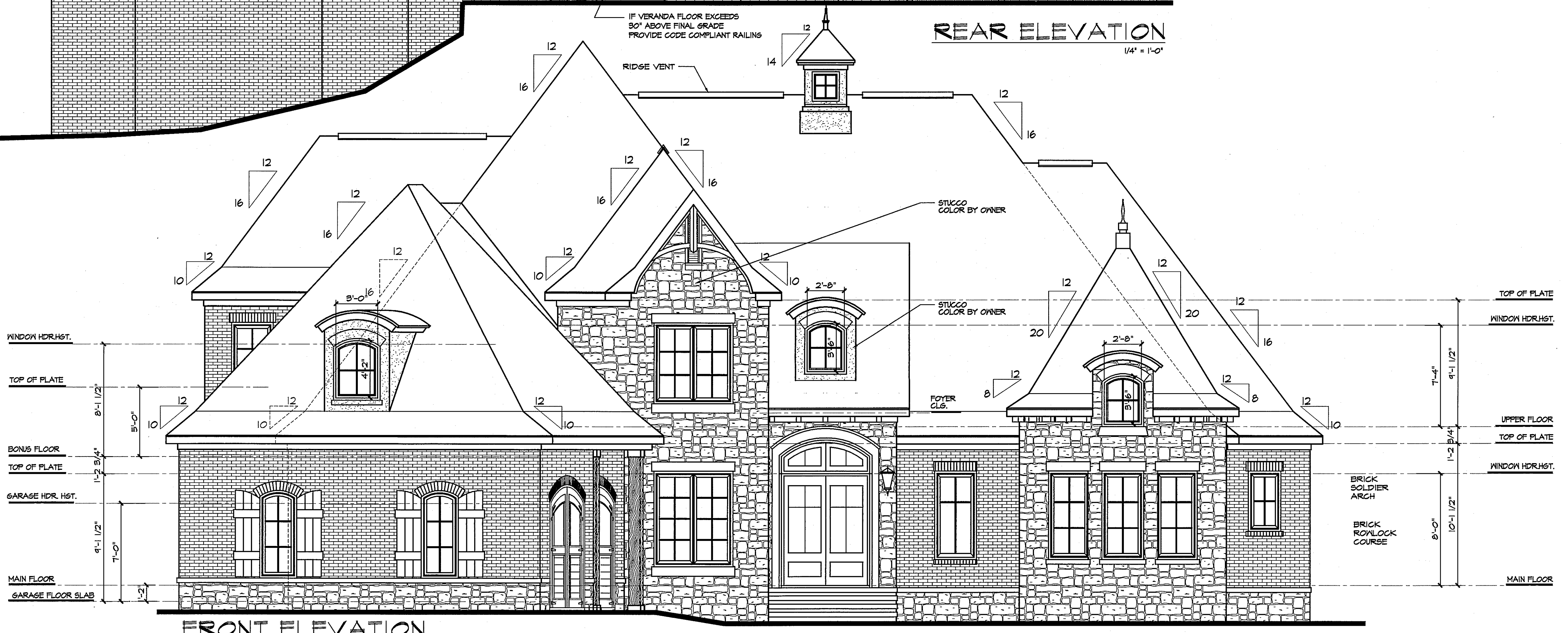
FRONT ELEVATION 1/4" = 1'-0"
