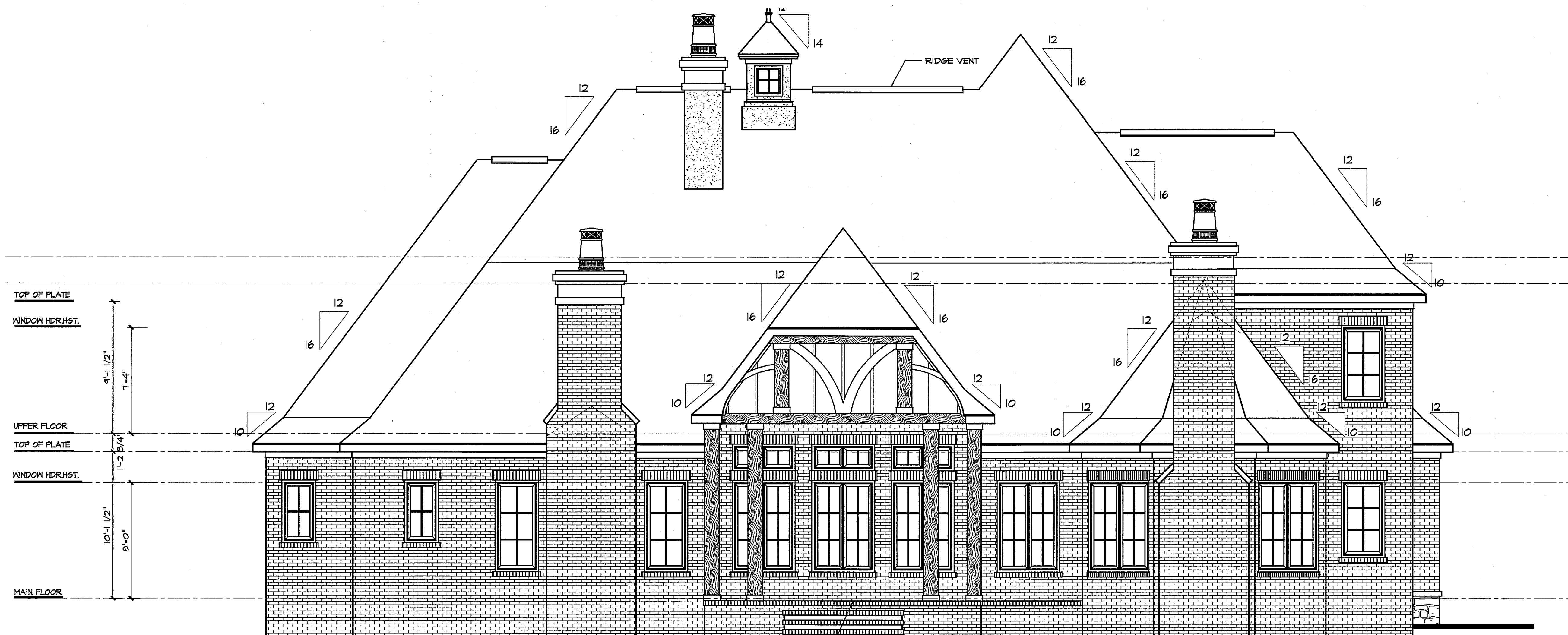
REAR ELEVATION 1/4" = 1'-0"
